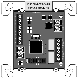
4090-9120 Six Point Module
