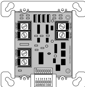
4090-9117 Addressable Power Isolator with IDNet Communications Control
