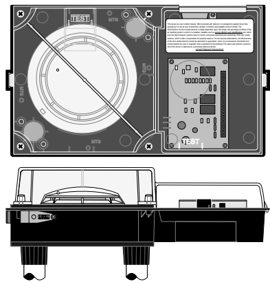
Duct Detector Housing, Front and Bottom View
